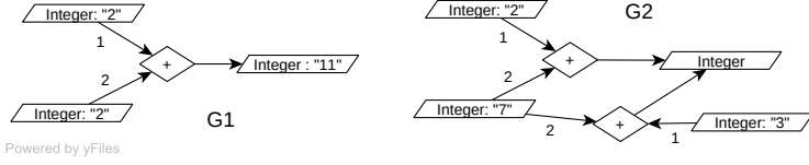
Fig. 4. Examples of D-graphs
