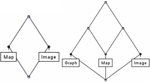
Fig. 6. Two simple lattices without attribute annotation corresponding to two sub-contexts. Left the lattice of concrete-iconic sign types (Image and Map), and right the extension of this lattice with the Graph type.
