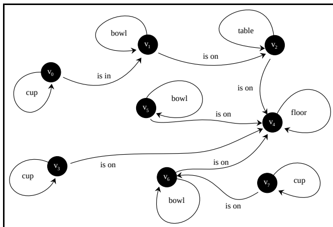
Fig. 2. Krahmer et al. scene digraph
