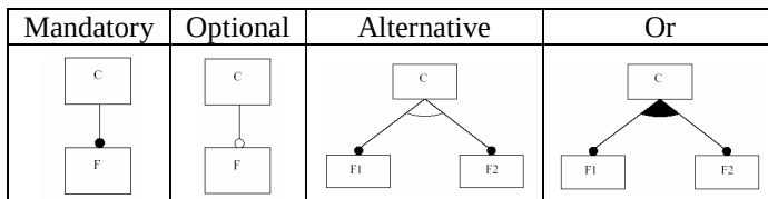
Fig. 3. Feature Modeling Node Notation [16]
