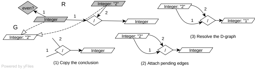
Fig. 7. Applying a D-rule on a D-graph
