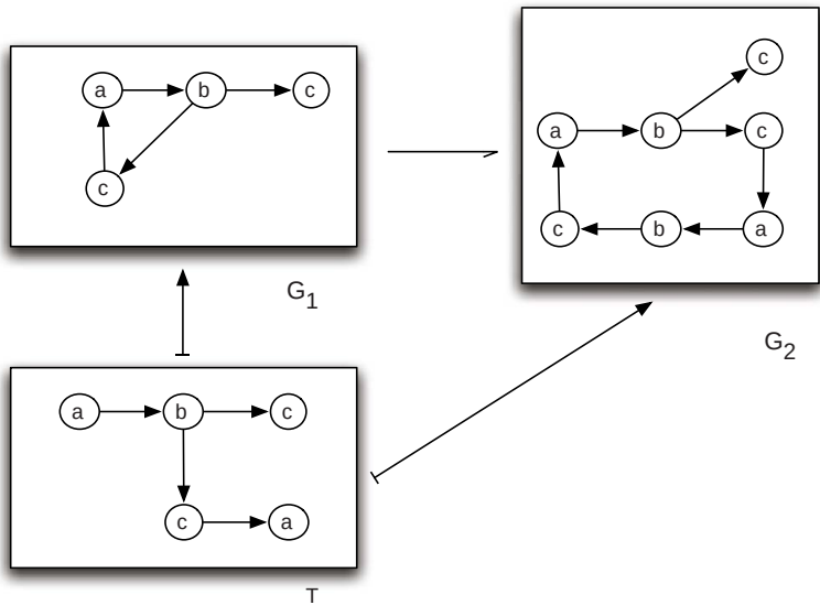
Fig. 2. AC-projection and interpretation
