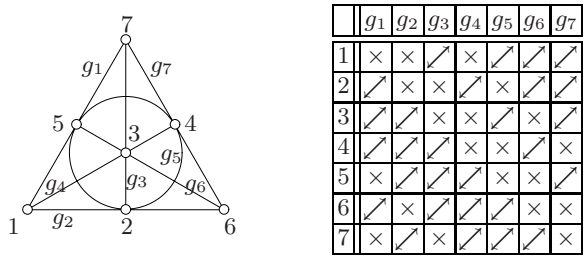
Fig. 3. The well known Fano plane with labelled points and lines, and its formal context representation
