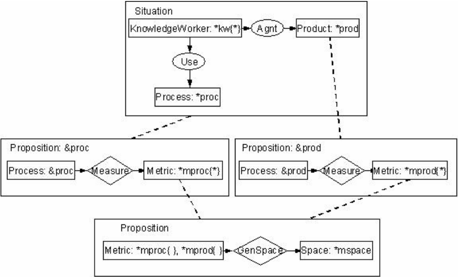
Fig. 2. Conceptual graphs, display form
